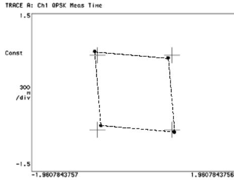
Figure 4-97 I/Q Quadrature Errors
