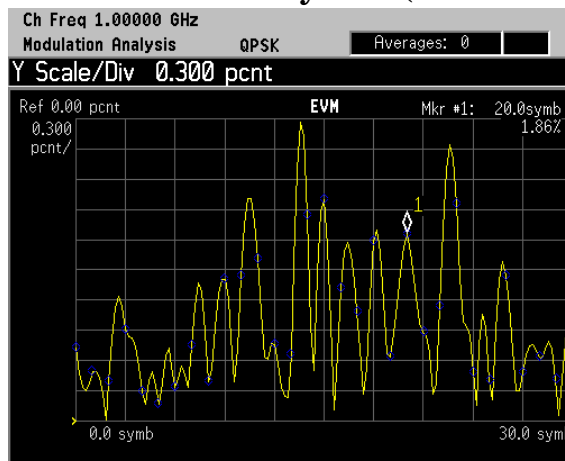
Figure 2-18 I/Q Error: EVM versus Symbol (Y-Axis Settings)
