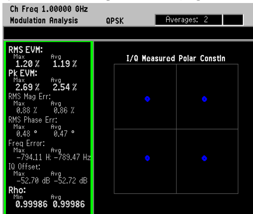
Figure 2-7 I/Q Measured Polar Graph (Left - Vector, Right - Constellation)
