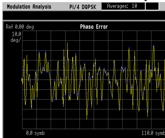
Figure 2-50 Phase Error Zoom View - Example of Uniform Noise
