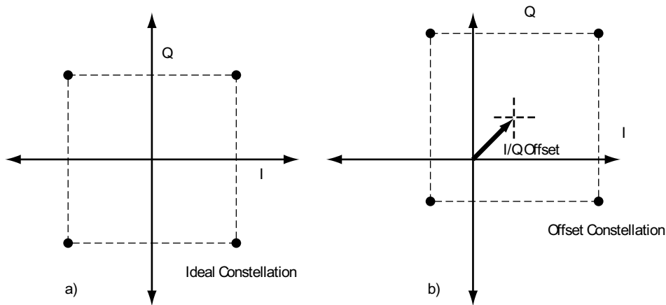
Figure 4-98 Ideal Versus I/Q Offset Constellation
