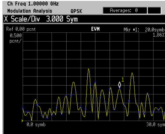
Figure 2-17 I/Q Error: EVM versus Symbol (X-Axis Settings)
