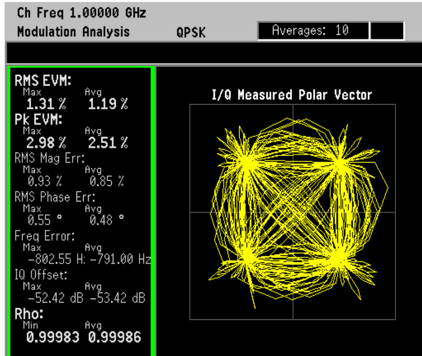
Figure 2-6 I/Q Measured Polar Graph - Polar Vector View
